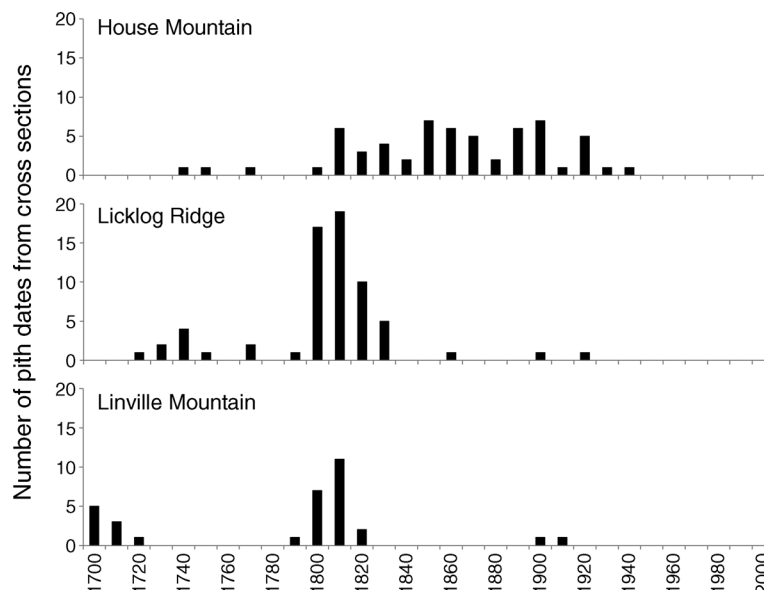
FIG. 4. The number of pith dates by decade for fire-scarred yellow pine cross sections for the years 1700–2000.
