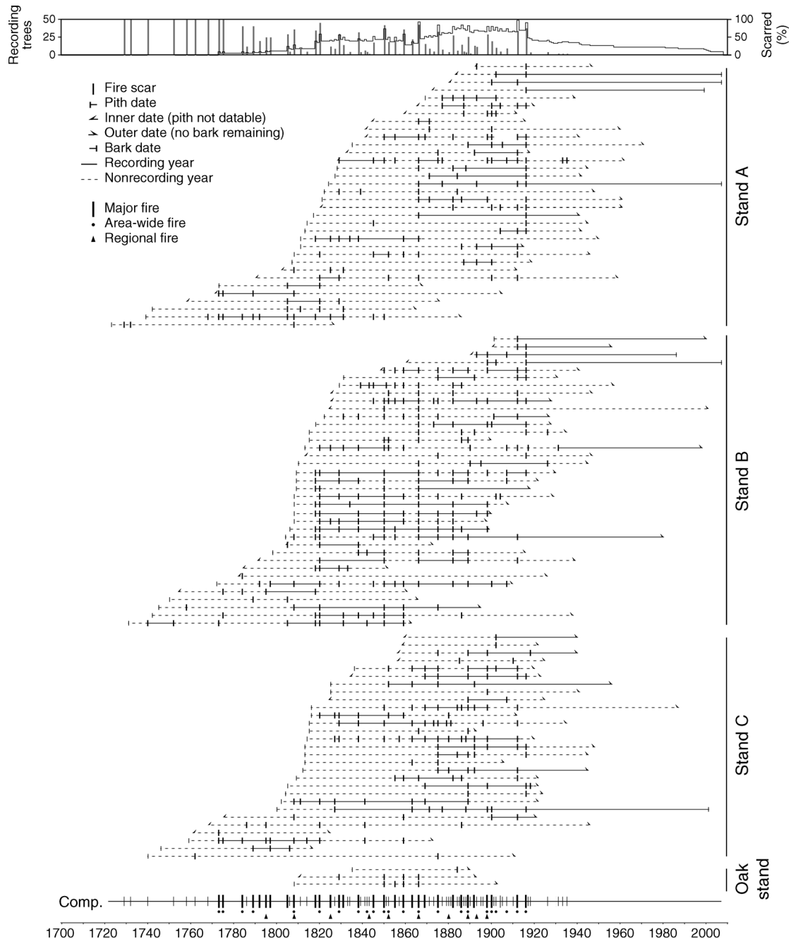
FIG. 6. Fire chronology for Licklog Ridge, Tennessee, showing the dated fire scars for each tree cross section, 1723–2008. See Fig. 5 for an explanation of the symbols used.
